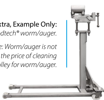
Cleaning trolley for worm/auger shown without worm/auger.
