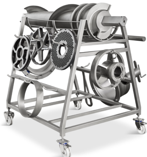
Heavy Duty designed worm/auger with sharp knife edge on hopper part of worm/auger to grab frozen blocks.
