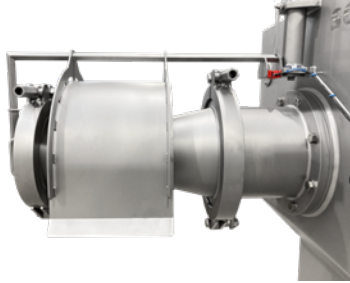
Extruder filter shown without safety cover.
