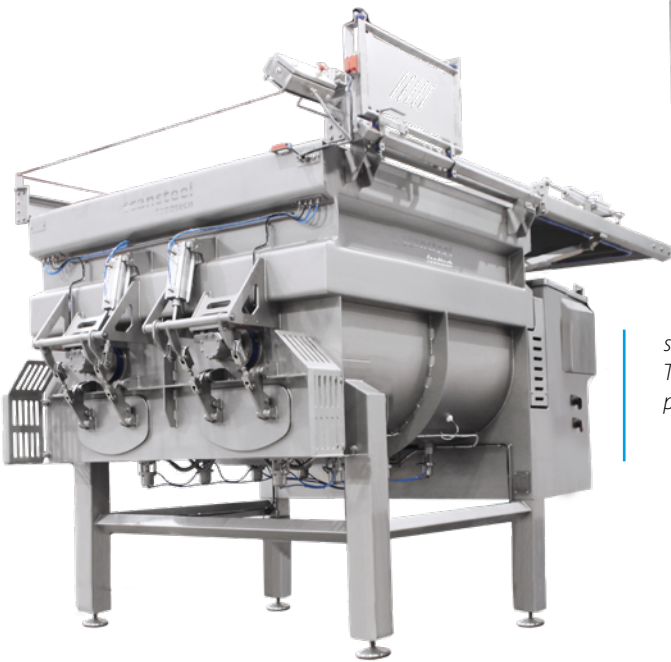
scansteel foodtech® Twin Shaft Mixer, TSM(V) positioning on floor.
